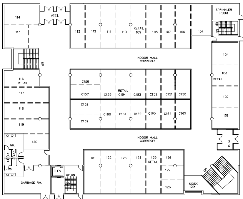
GROUND FLOOR PLAN SCALE 1:200
